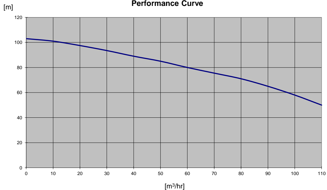
Performance Curve
