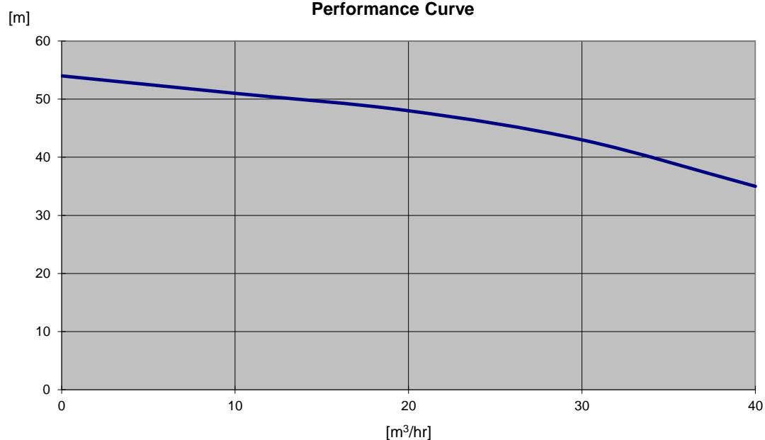
Performance Curve
