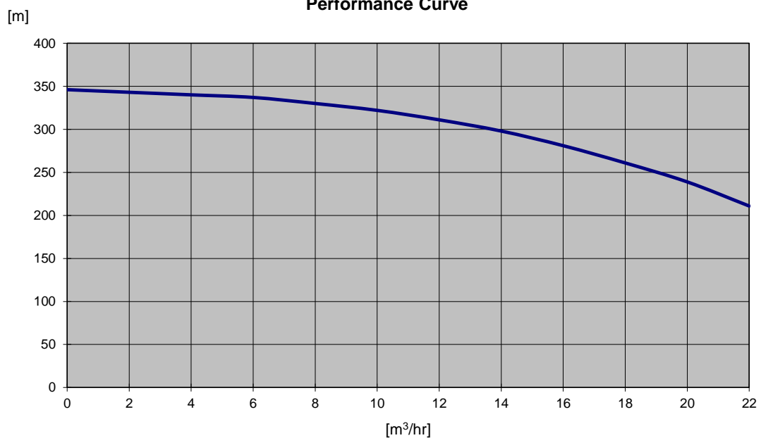
Performance Curve
